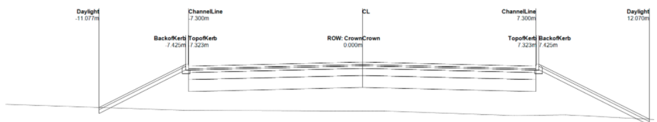
A650 Alignment
