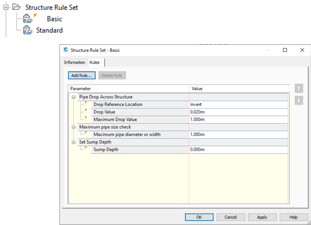
Rules assigned to the 'Basic' Structure Rule Set
